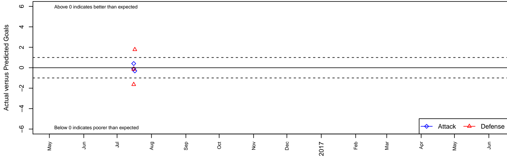
Beach FC Long Beach B99 Dots are actual minus expected GF (blue circles) and GA (red triangles). Blue line is smoothed change in attack strength. Red is smoothed change in defense strength.
